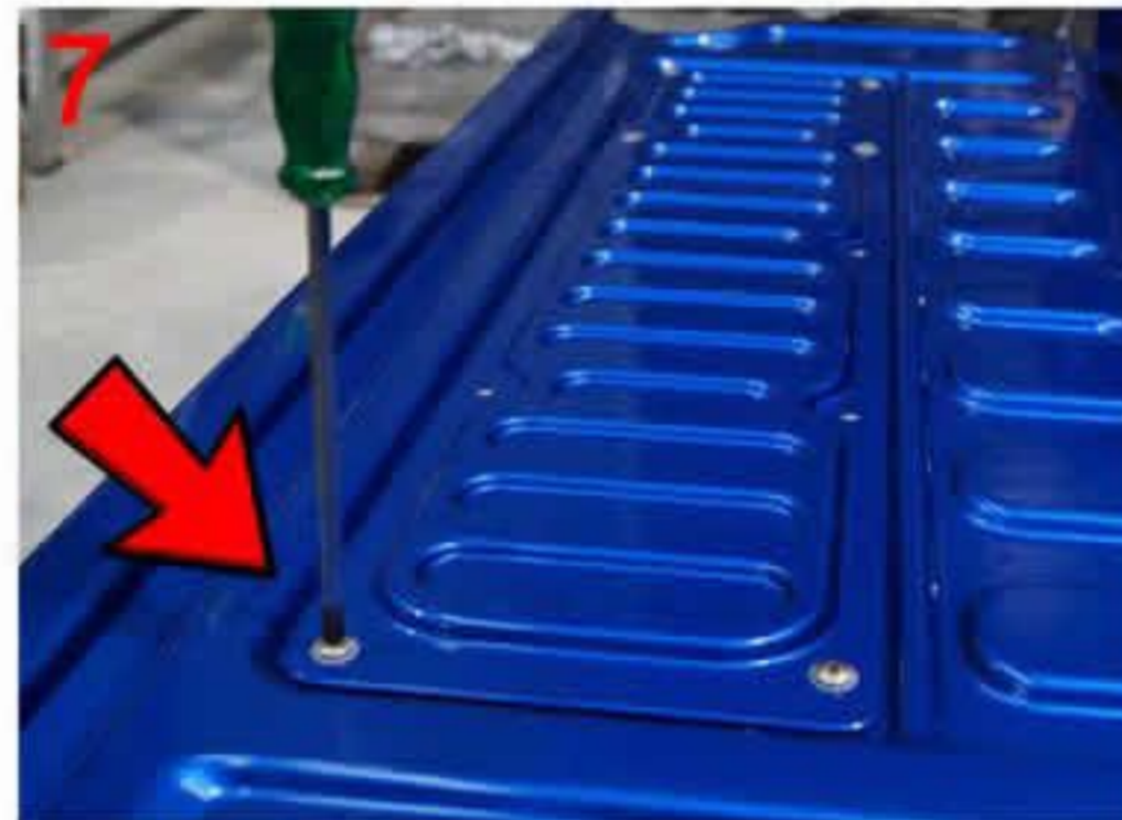
7: Remove tailgate access panel bolts as shown
