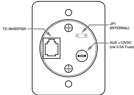
Figure 3.1 - Rear Panel Connections
