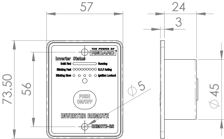
Figure 2.1 - REMOTE-RS Dimensions
